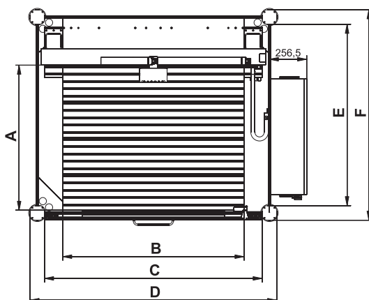
FlatCom with sub-frame and hood
