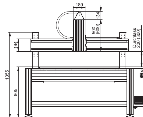
FlatCom with sub-frame, without hood
