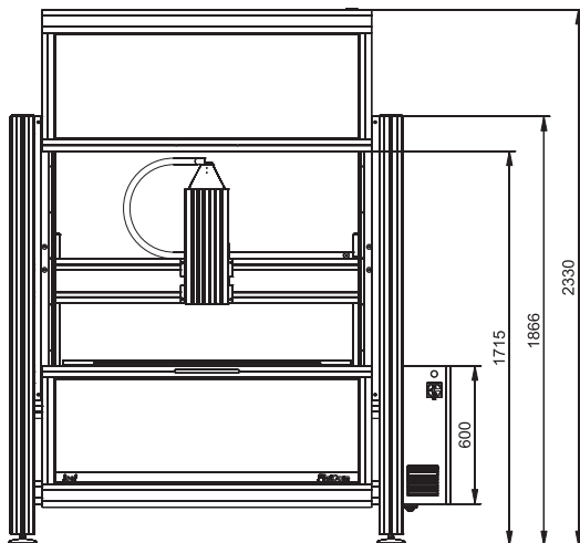
FlatCom with sub-frame and hood
